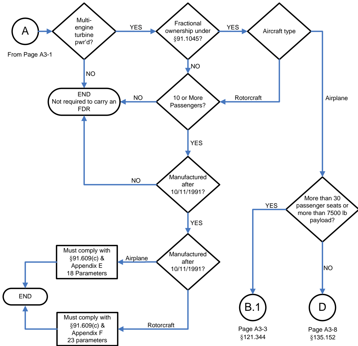
FIGURE 3-2. PART 91 FLIGHT RECORDER PARAMETER REQUIREMENTS § 91.609
